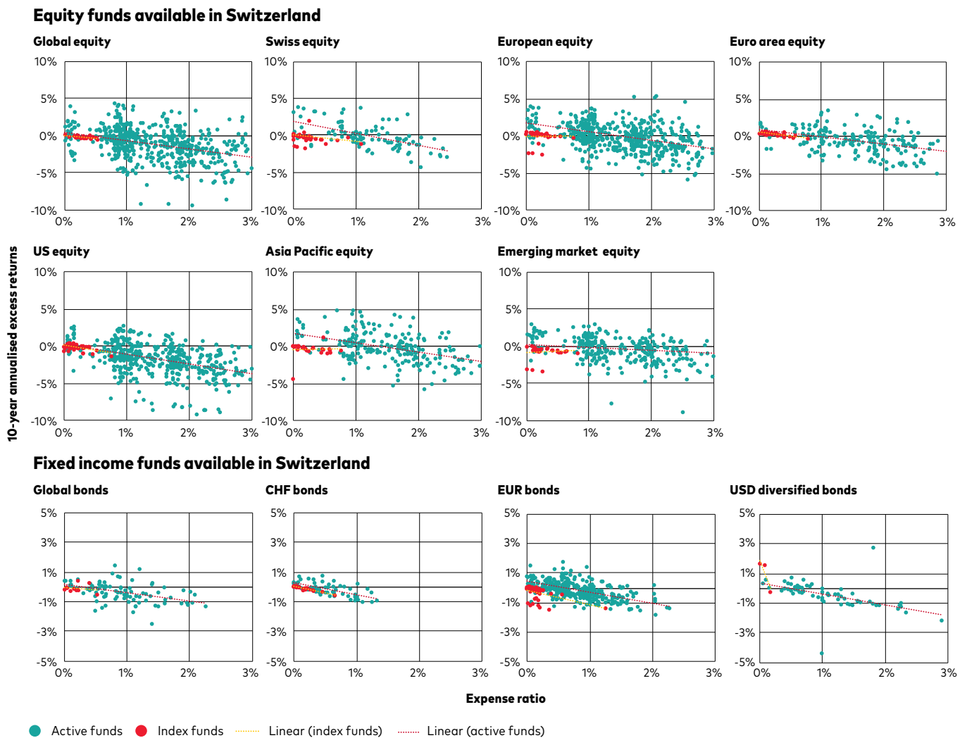
FIGURE 4. Higher expense ratios were associated with lower excess returns
