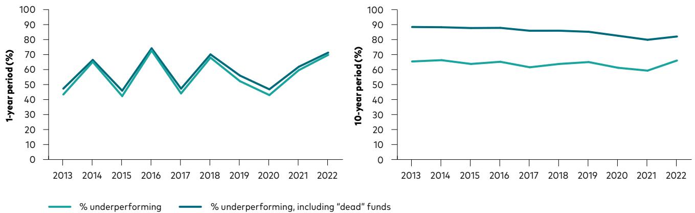
FIGURE 7. Percentage of active equity funds available in Switzerland underperforming over rolling periods versus prospectus benchmarks
